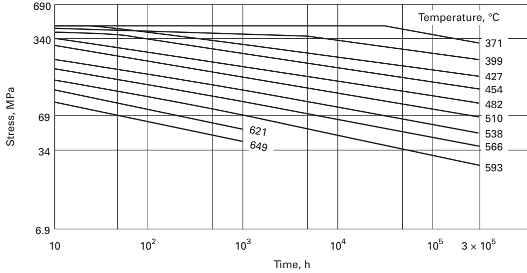
Figure E-100.7-4 Expected Minimum Stress-to-Rupture Values, MPa, 2¼Cr-1Mo
