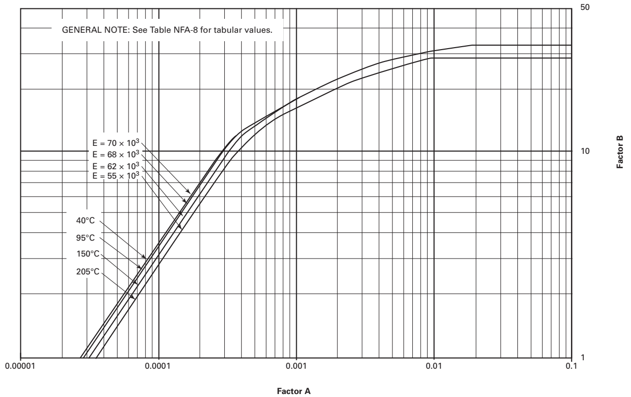
Figure NFA-8 Chart for Determining Shell Thickness of Components Under External Pressure Developed for Aluminum Alloy 5052 in 0 Temper
