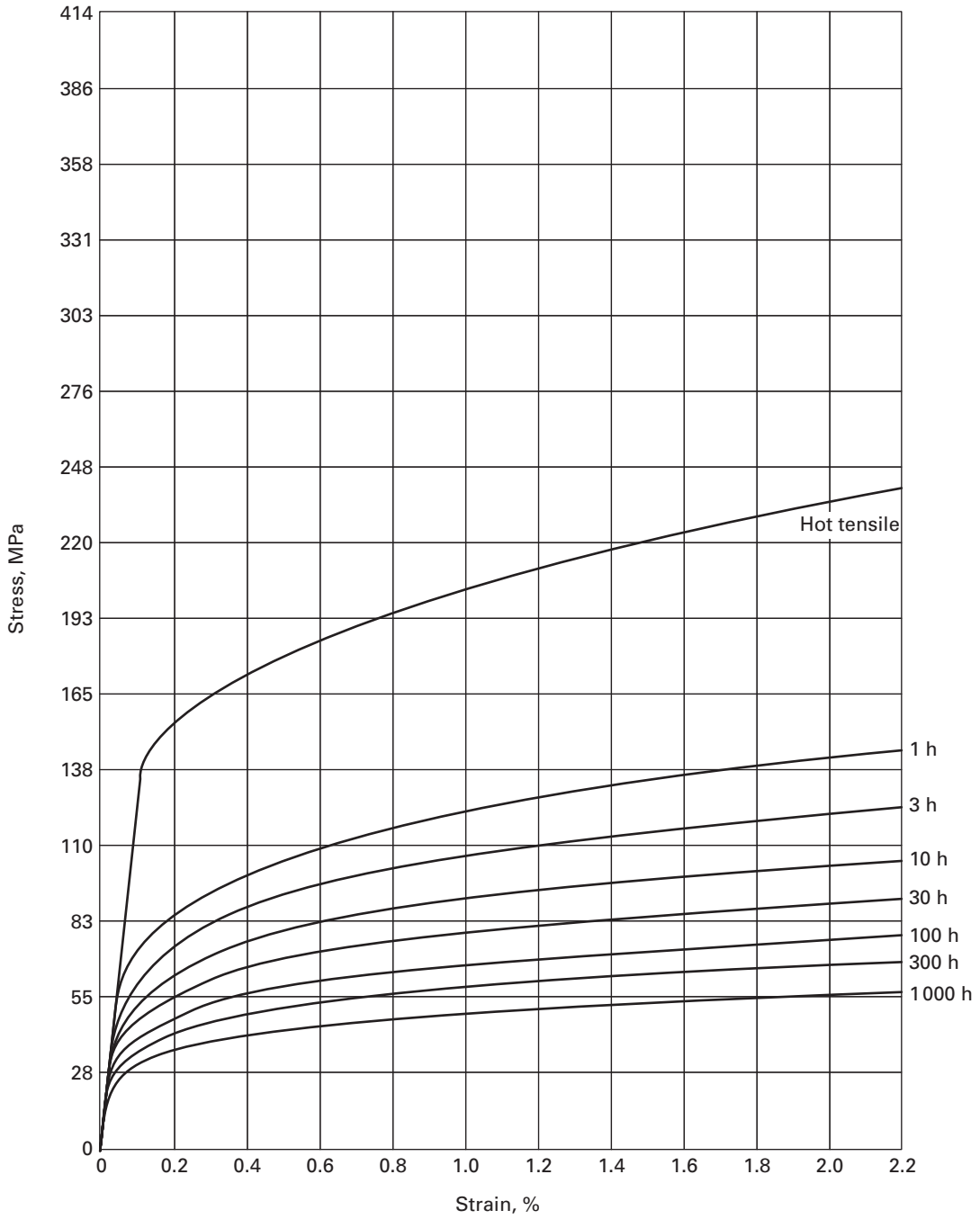
Figure E-100.21-10 Average Isochronous Stress-Strain Curves for Annealed 2 \frac{1}{4} Cr-1Mo at 621°C
